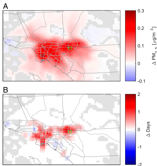
Fig. 4. (A) Change in annual average PM_{2.5} concentrations (scenario IV – scenario I). The green circle indicates the location of the highest annual PM_{2.5} measured DVs in the basin. Seasonal differences in PM_{2.5} are presented in SI Appendix, Fig. S34 . (B) Change in the number of 24-h PM_{2.5} federal standard ( 35 \mu\text{g}\cdot\text{m}^{-3} ) exceedance days in a year (scenario IV – scenario I). Gray hashed cells indicate that differences are not statistically significant ( P > 0.05 ). Image represents 3 \times 3 -cell moving average.
