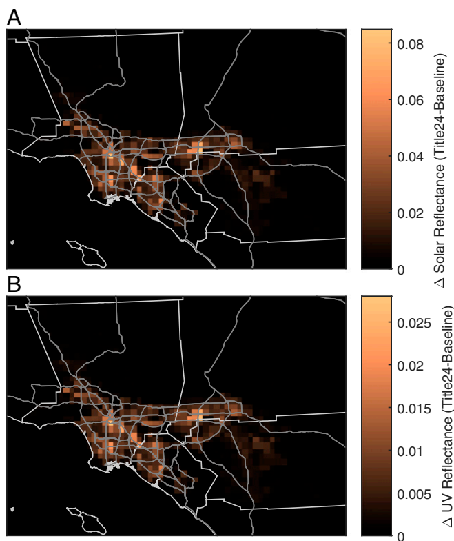
Fig. 1. (A) Change in SR (Title24 – baseline) used for WRF simulations. (B) Maximum possible change in UVR (Title24 – baseline) used for CMAQ simulations.
