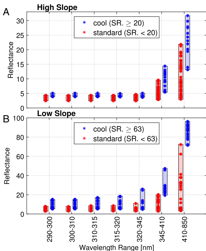
Fig. 2. Range of wavelength-dependent reflectance of cool and standard roofing materials for high-slope (A) and low-slope (B) applications.
