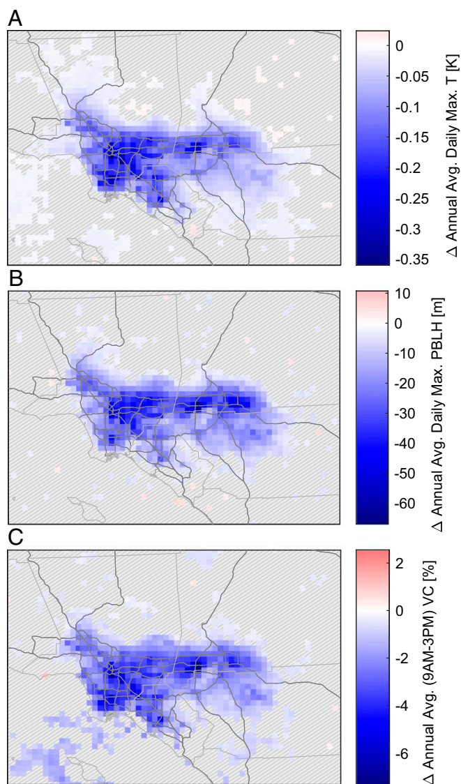
Fig. 3. (A) Change in annual average daily max temperatures (Title24 – baseline). (B) Change in annual average daily maximum PBLH. (C) Change in annual average VC calculated between 9 AM and 3 PM. Gray hashed cells indicate that differences are not statistically significant ( P > 0.05 ).
